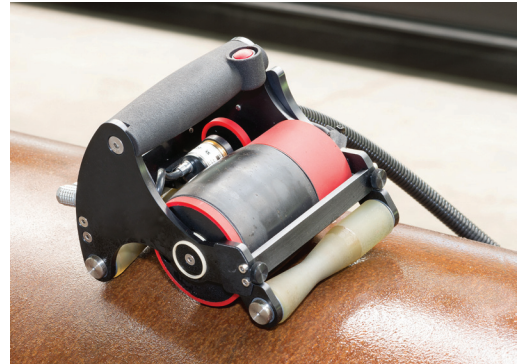
Roller probe for longitudinal testing of bars and tubes
