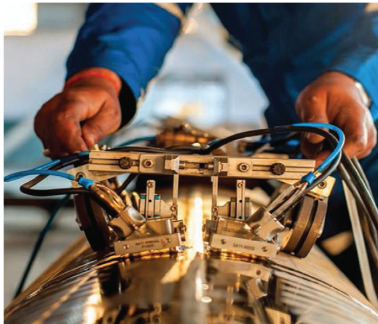
Scanner for manual testing of longitudinal tube welds with position encoder and suspensions for 2 Phased Array probes and 2 TOFD probes
